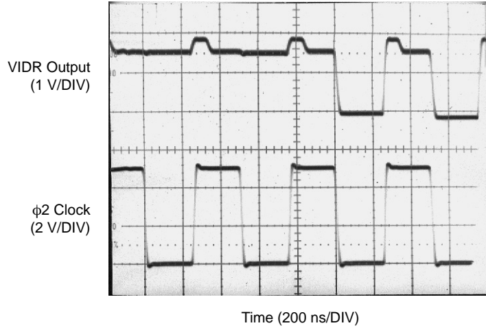
Figure 4. Output Waveforms
