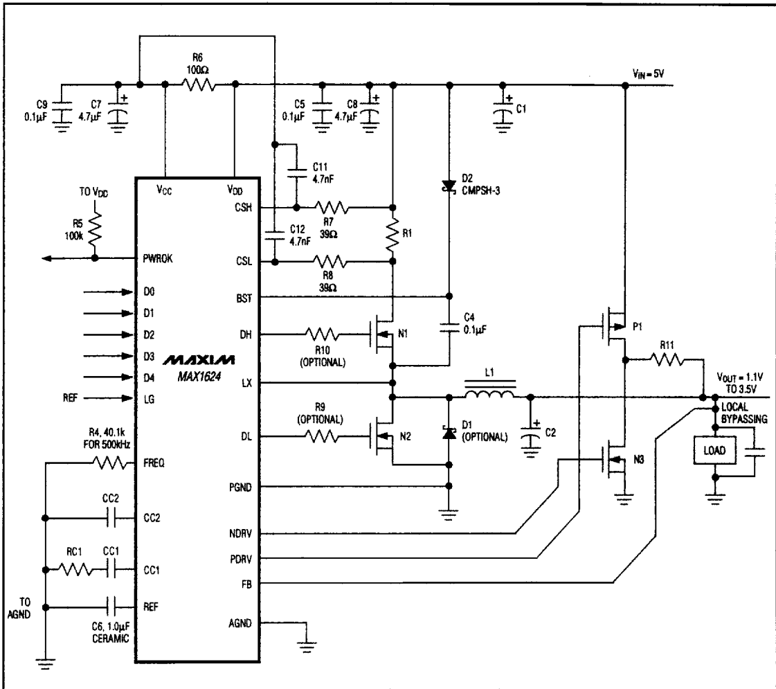
Figure 1. MAX1624 Standard Application Circuit
