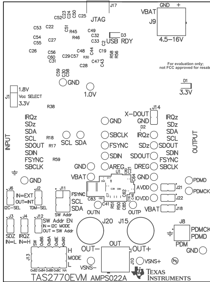
Figure 12. PCB: Top Silkscreen
