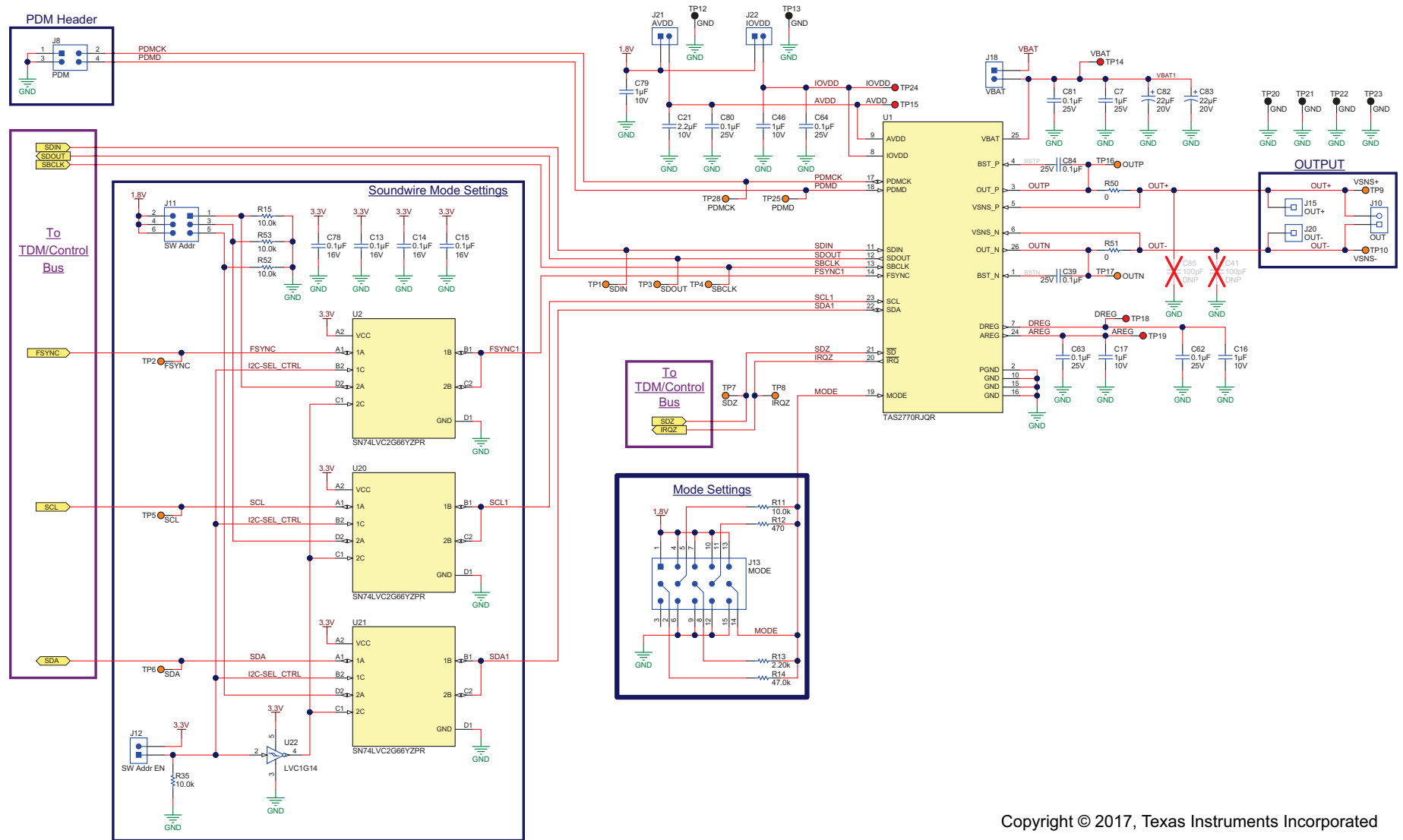
Figure 10. Schematic: TAS2770 Channel 1 Control
