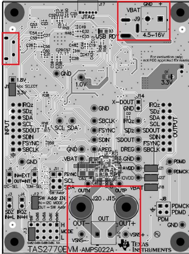
Figure 1. TAS2770EVM Stereo Configuration
