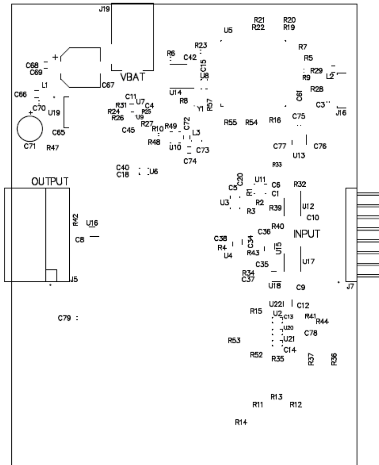
Figure 19. PCB: Bottom Silkscreen
