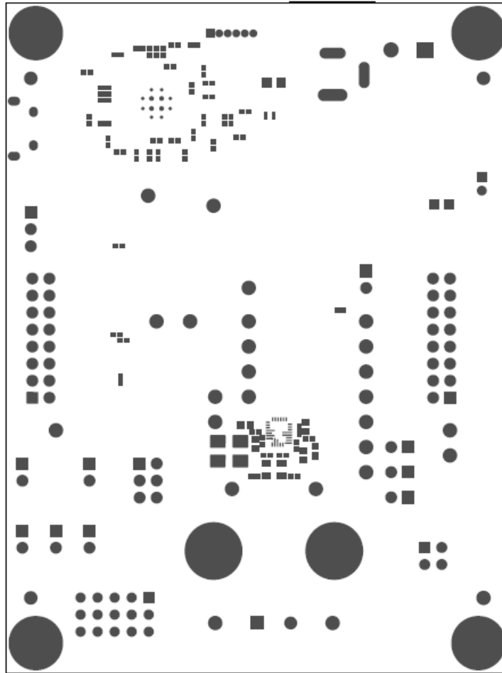
Figure 13. PCB: Top Solder Mask
