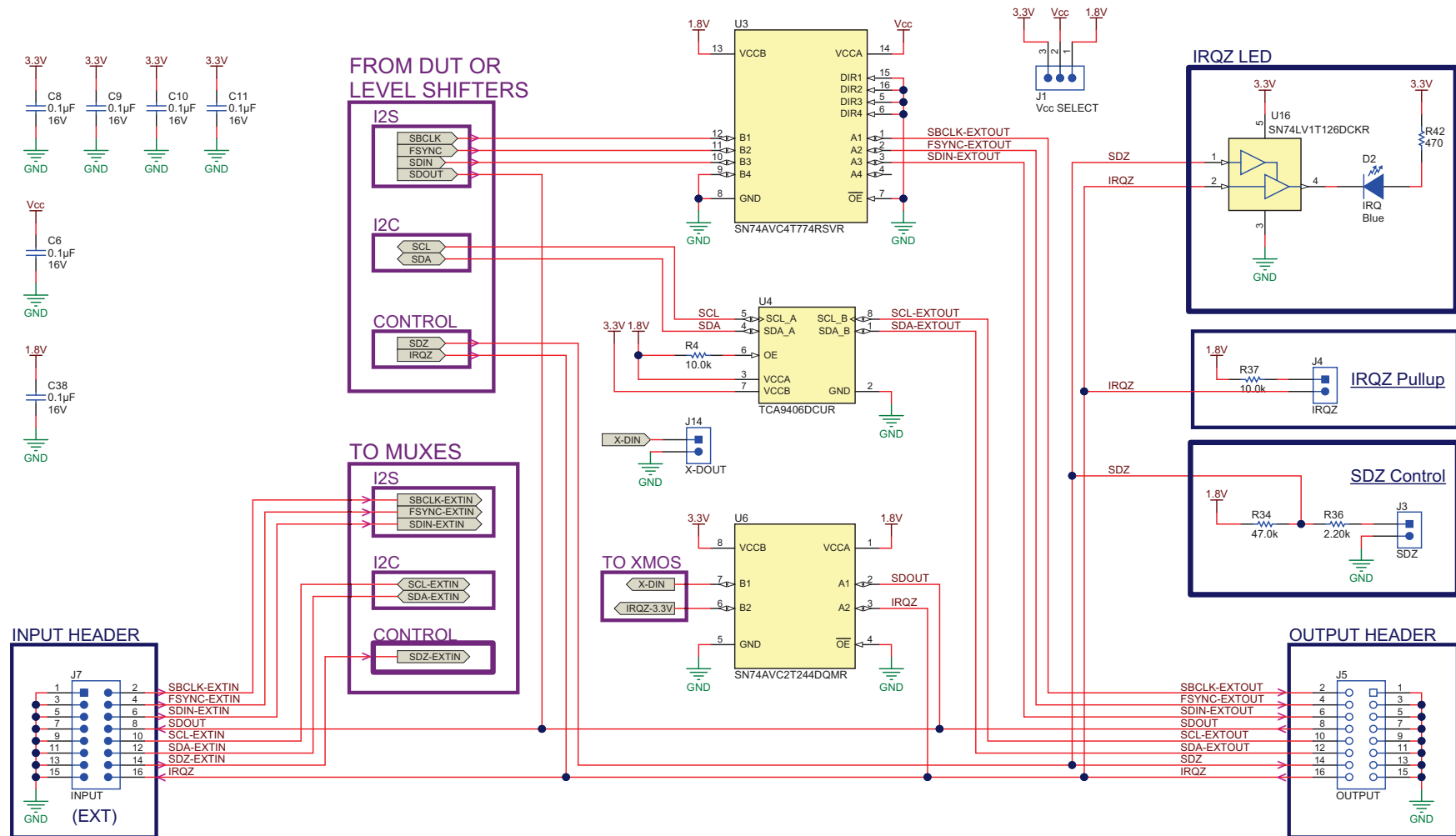
Figure 9. Schematic: External Input and Output Routing
