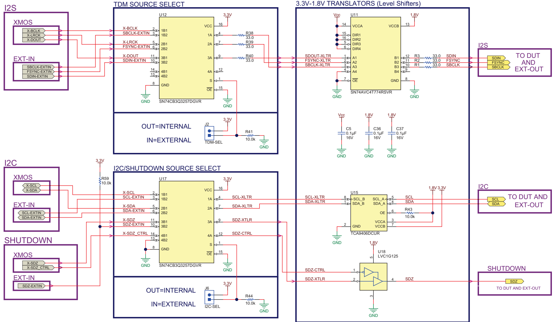
Figure 8. Schematic: Input Multiplexing and Level Shift
