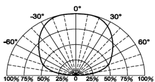
Fig.6 Directive Radiation
