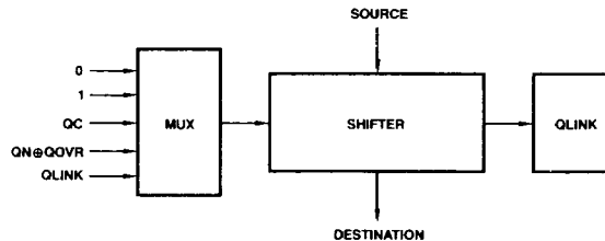
Figure 3. Shift-Down Function
