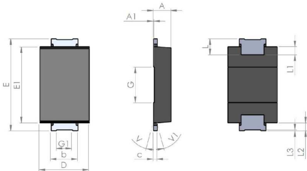
Figure 17. SMA Flat Notch package outline
