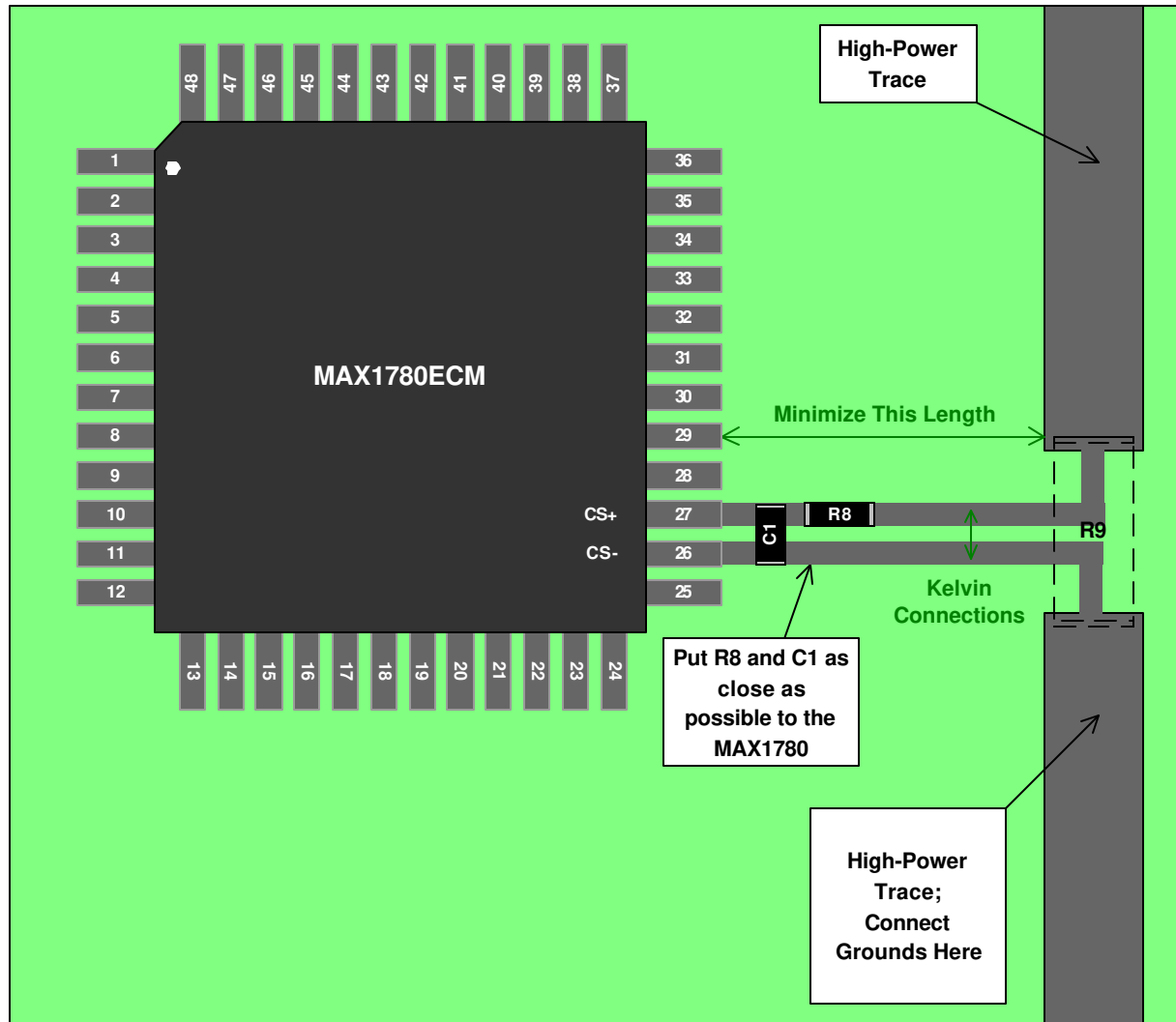
Figure 29, Layout Recommendation For Current Sense Inputs
