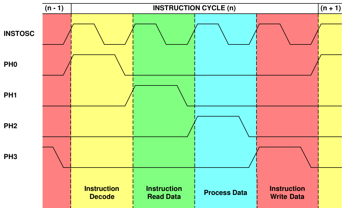
Figure 4, Instruction Cycle Phase Clocks
