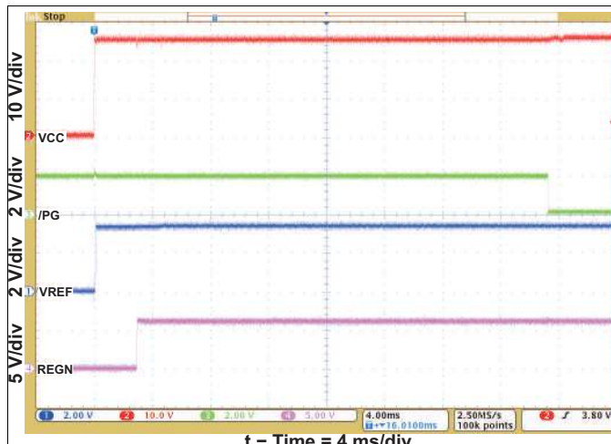
Figure 1. REF, REGN, and \overline{PG} Power Up (CE = 1)
