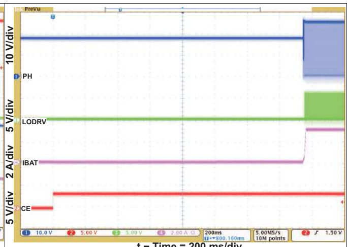
Figure 2. Charge Enable
