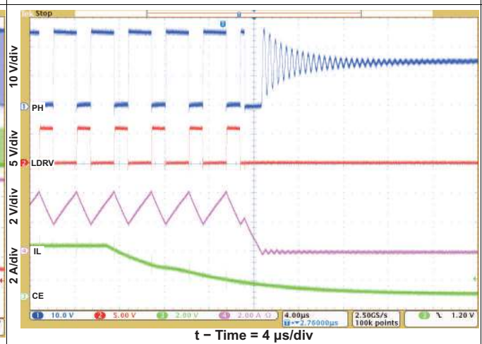
Figure 4. Charge Disable
