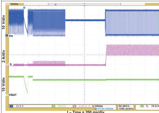
Figure 9. Battery Insertion
