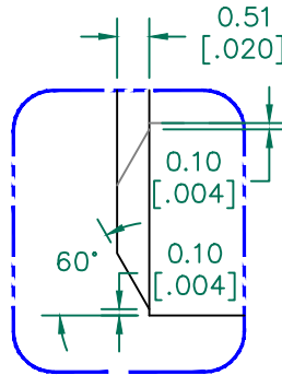
DETAIL "A" CHAMFER SCALE=8:1
