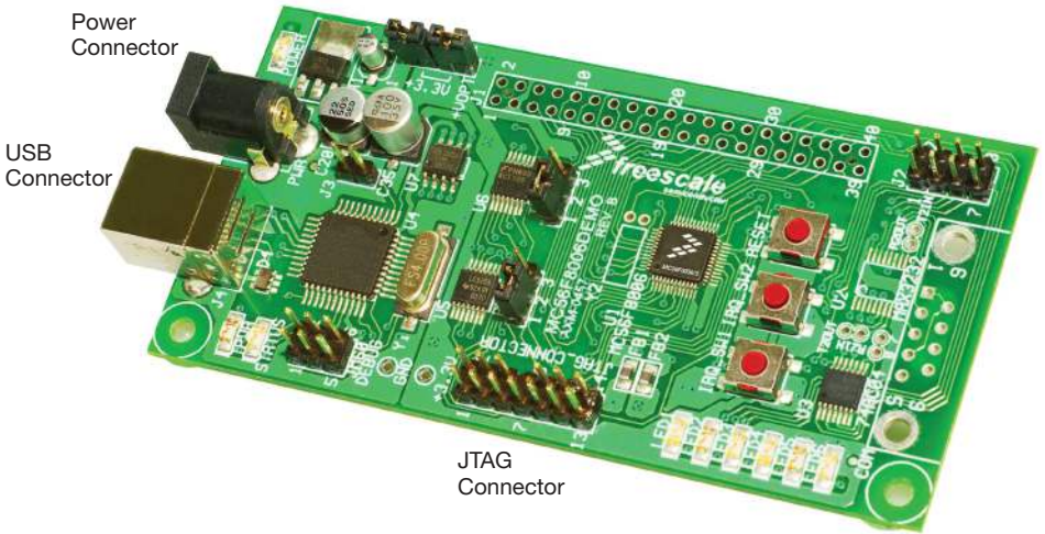
Figure 1. MC56F8006DEMO
