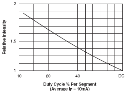
Fig. 5 Luminous Intensity vs. Duty Cycle
