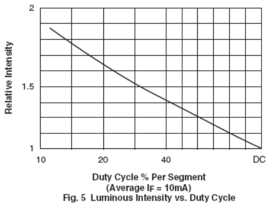
Fig. 5 Luminous Intensity vs. Duty Cycle
