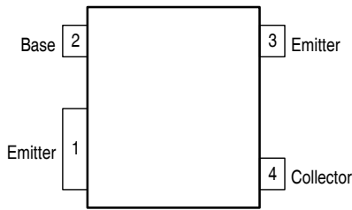
Figure 1. Pin Connections
