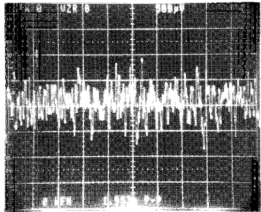
A_{\text{CL}} = 25,000\text{V/V} Horizontal Scale = 1s/Div. Vertical Scale = 0.002\mu\text{V/Div} , E_{\text{N}} = 0.08\mu\text{V}_{\text{p-p RTI}}
