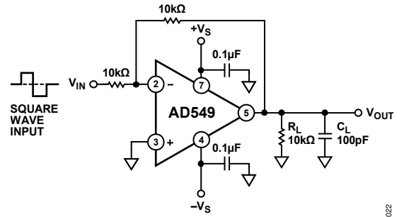
Figure 22. Unity-Gain Inverter
