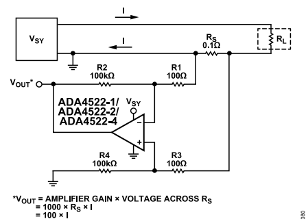
Figure 84. Low-Side Current Sensing Circuit
