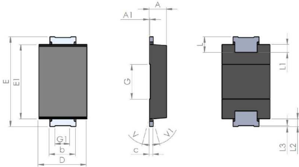
Figure 20. SMA Flat Notch package outline
