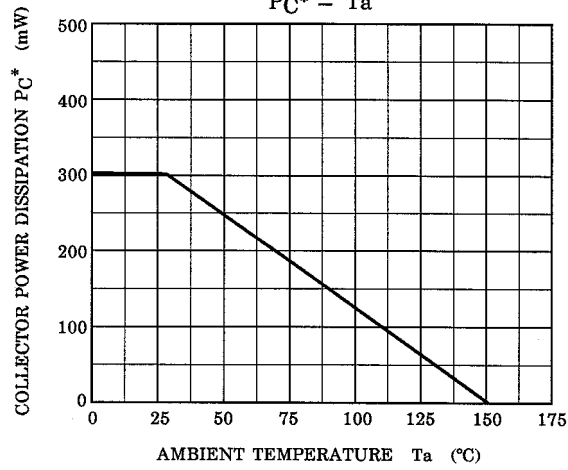
P_C^* - T_a
