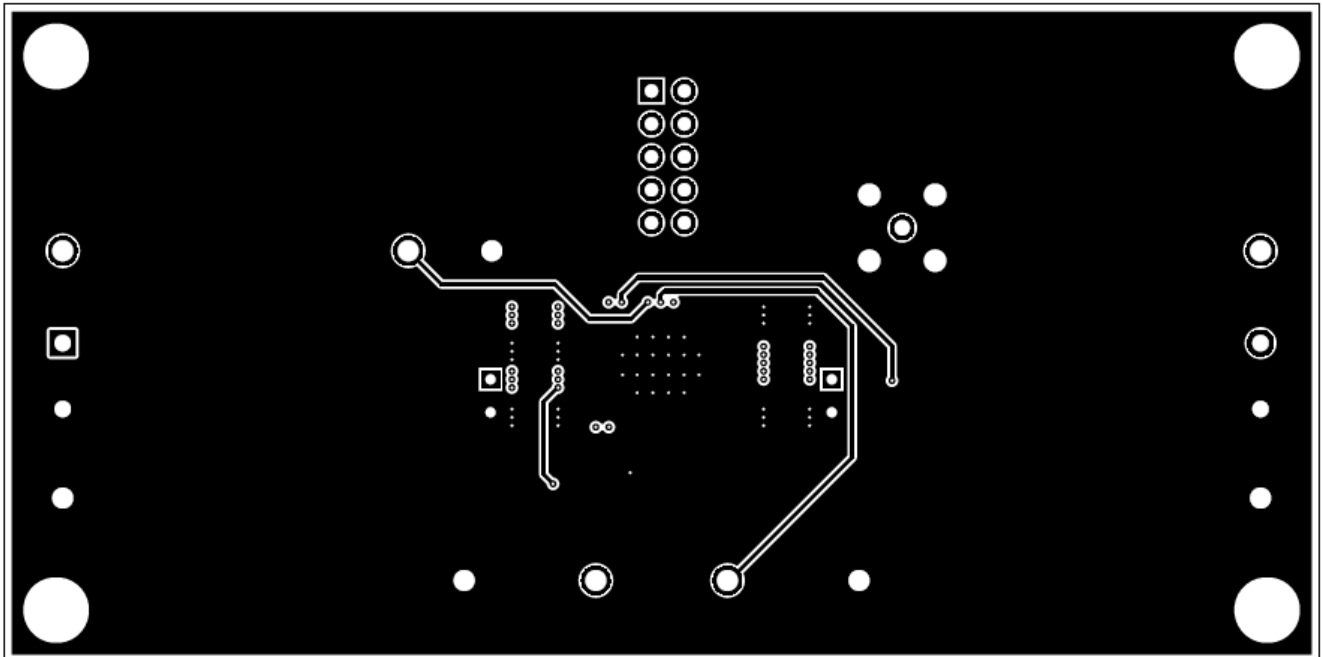
Figure 8-4. Layer 2 Copper
