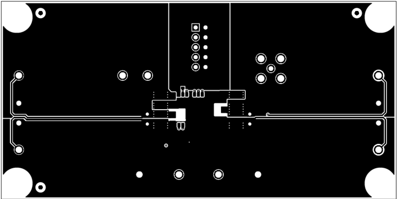
Figure 8-3. Top Copper
