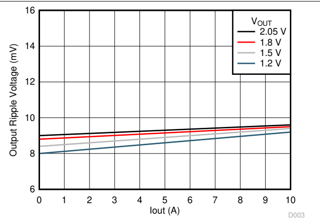
Figure 5-4. TPSM84A22EVM Output Voltage Ripple
