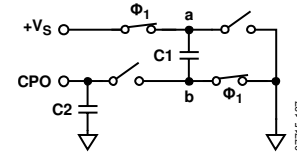
Figure 30. Charging Cycle
