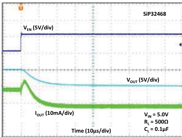
Fig. 35 - Turn-off Time
