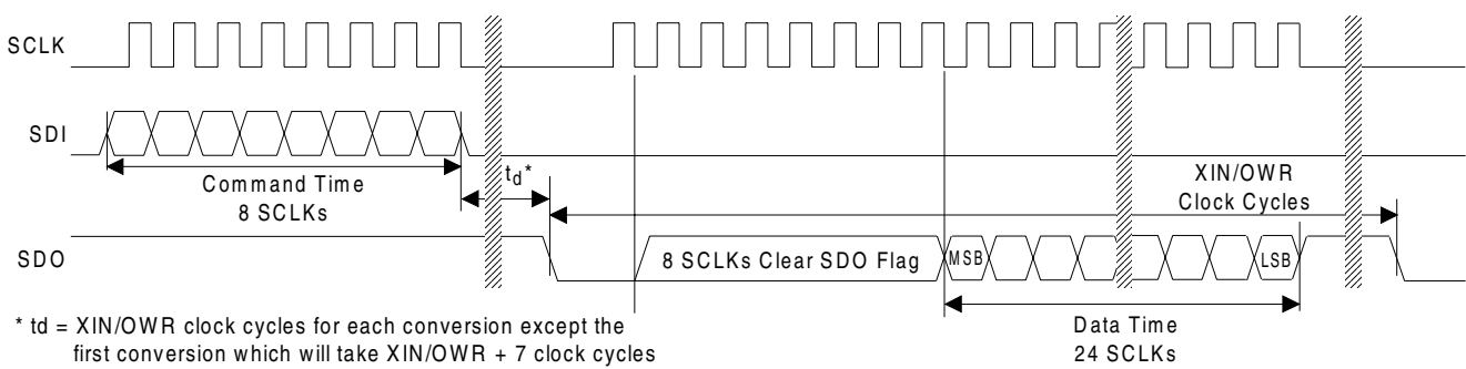
SDO Continuous Conversion Read (PF bit = 1)
