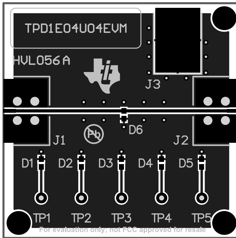
Figure 3. TPD1E04U04EVM Top Layer and Silkscreen
