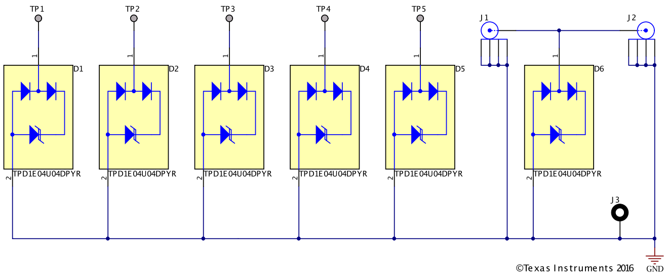
Figure 4. TPD1E04U04EVM Schematic
