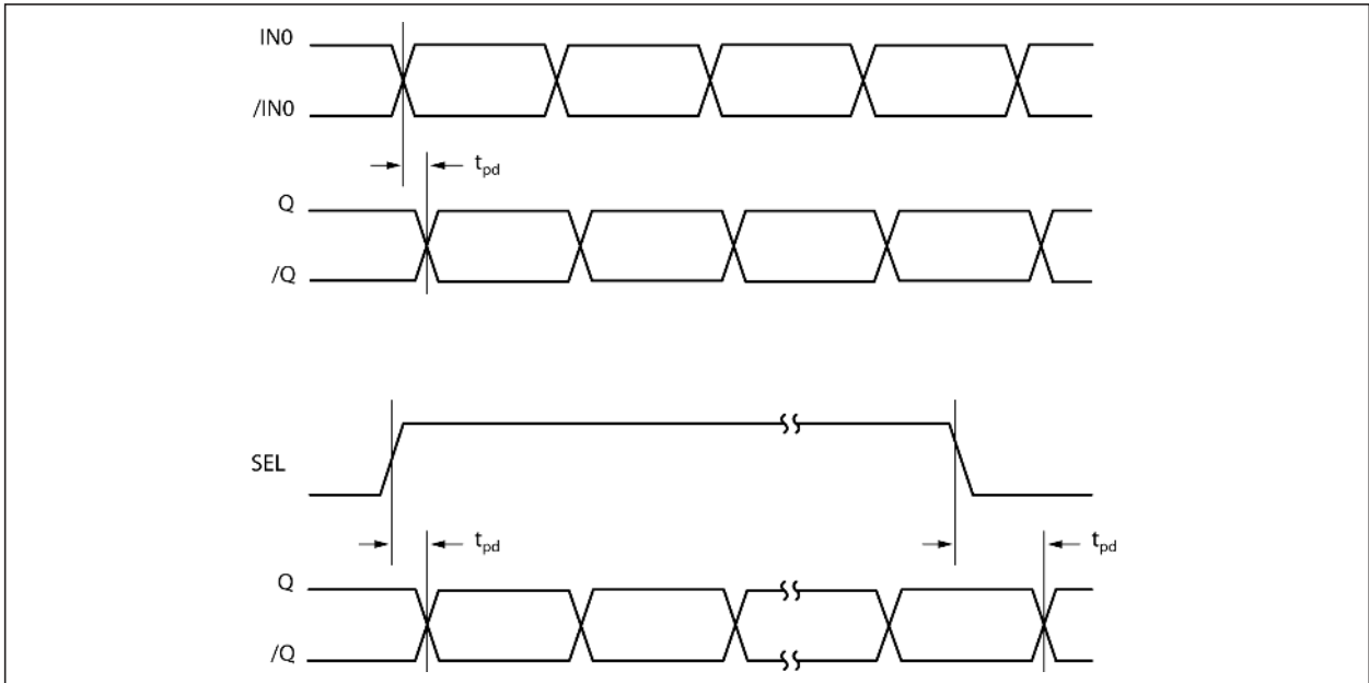
FIGURE 3-1: Propagation Delay.
