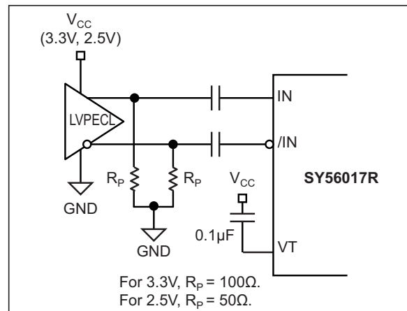
FIGURE 4-4: LVPECL Interface (AC-Coupled). For 3.3V, R P = 100Ω. For 2.5V, R P = 50Ω.
