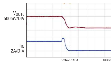
FIGURE 46 CIRCUIT, 12VIN, 30A LOAD ON V_{OUT0} PRIOR TO APPLICATION OF SHORT-CIRCUIT USE HIGH RANGE OF I LIMIT SYSTEM SHORT-CIRCUIT USING LOW IMPEDANCE COPPER ACROSS OUTPUT (HARD SHORT)
