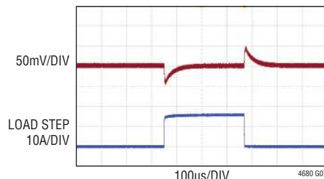
FIGURE 46 CIRCUIT, 12V TO 1.8V, FREQ = 500kHz C_{OUT} = 470\mu\text{F} \times 2 POSCAP, 100\mu\text{F} \times 4 CERAMIC R_{COMP} = 17\text{k} , EA-GM = 3.69ms, COMP_{na} = 3.3\text{nF} , COMP_{nb} = 68\text{pF} I_{LIM} LOW, V_{OUT} RANGE LOW
