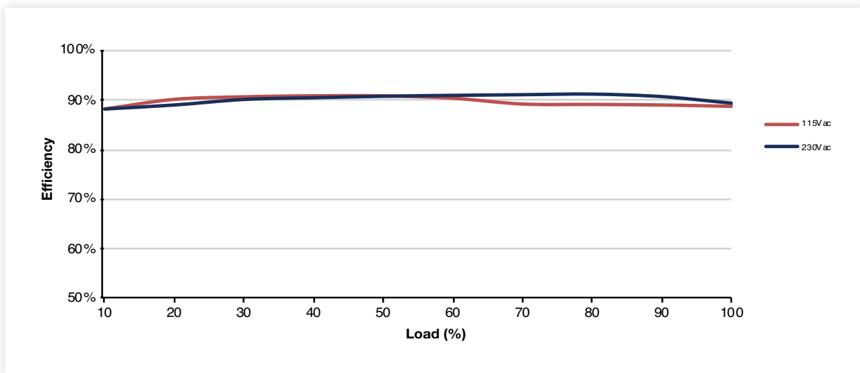
VCB60US12
