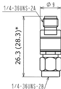
SMA Type (Plug - Jack) AT-100V
