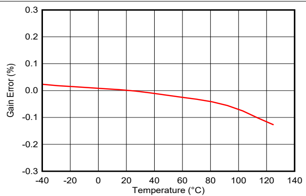
Figure 9-3. Gain Error vs Temperature (ADC1A, ADC1B)
