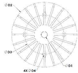
100 mm Diameter Heat Sinks
