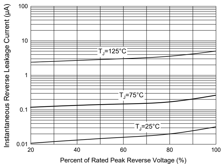
Fig. 3 - Reverse Leakage Characteristics
