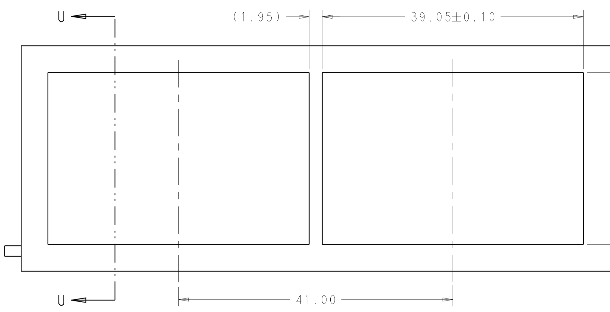
RECOMMENDED PANEL CUTOUT AND PC BOARD, PANEL POSITION SCALE 3:1
