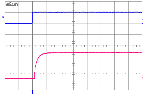
Figure 7. Turn-on transient at full rated load current (resistive) plus 10,000\ \mu\text{F} at V_{in} = 48\text{ V} , triggered via ON/OFF pin. Top trace: ON/OFF signal (5 V/div.). Bottom trace: Output voltage (0.5 V/div.). Time scale: 5 ms/div.
