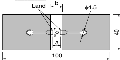
Fig.1 (in mm)
