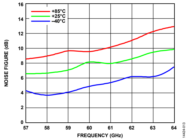
Figure 13. Noise Figure vs. Frequency over Temperature
