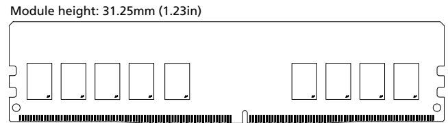
Figure 2: 288-Pin UDIMM (R/C D2)
