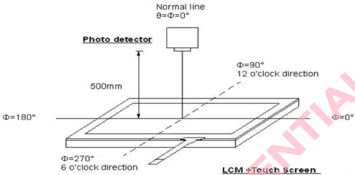
Fig. Optical measurement system setup
