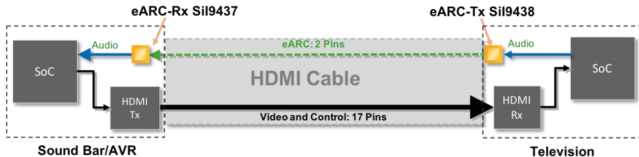
Figure 3: Lattice Sil9437 and Sil9438 Solutions for eARC
