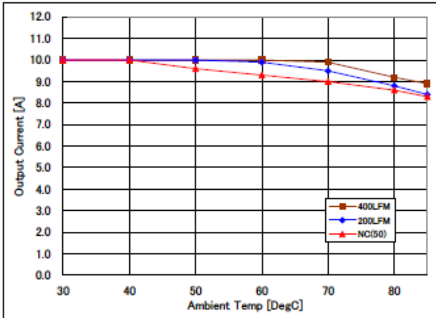
Fig-2.5V-1: Available load current vs. ambient temperature and airflow rates for Vout=2.5V with Vin=12.0V. Maximum component temperature \leq 120°C
