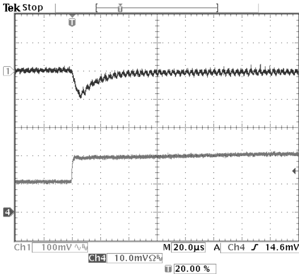
Fig-1.2V-6: Output voltage response for V_{out}=1.2V to positive load current step-change from 5A to 10A with slew rate of 5A/us at V_{in}=12.0V . C_o=47\mu F \times 2 ceramic. Top trace: output voltage (100mV/div.) Bottom trace: load current (5A/div.) Time scale: 20us/div.
