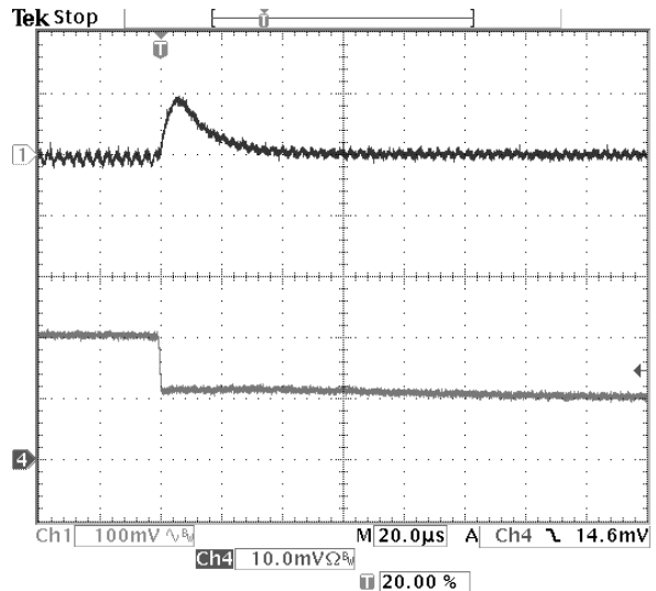
Fig-1.5V-7: Output voltage response for V_{out}=1.5V to positive load current step-change from 10A to 5A with slew rate of -5A/us at V_{in}=12.0V . C_o=47\mu F \times 2 ceramic. Top trace: output voltage (100mV/div.) Bottom trace: load current (5A/div.) Time scale: 20us/div.
