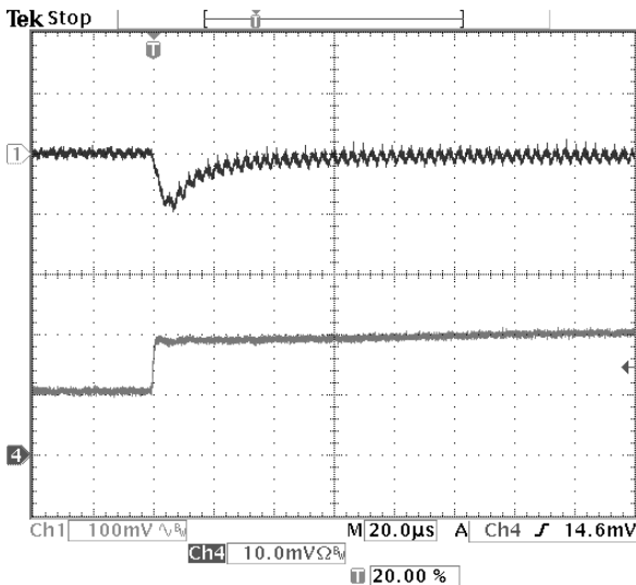
Fig-1.5V-6: Output voltage response for V_{out}=1.5V to positive load current step-change from 5A to 10A with slew rate of 5A/us at V_{in}=12.0V . C_o=47\mu F \times 2 ceramic. Top trace: output voltage (100mV/div.) Bottom trace: load current (5A/div.) Time scale: 20us/div.
