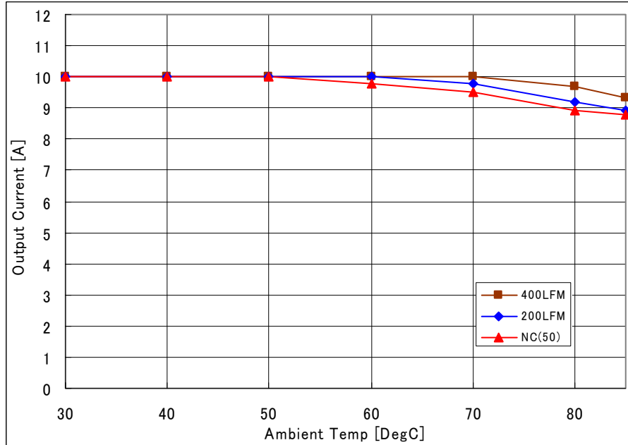
Fig-1.0V-1: Available load current vs. ambient temperature and airflow rates for Vout=1.0V with Vin=12.0V. Maximum component temperature \leq 120^{\circ}\text{C}
