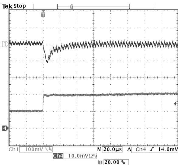
Fig-3.3V-6: Output voltage response for V_{out}=3.3V to positive load current step-change from 5A to 10A with slew rate of 5A/us at V_{in}=12.0V . C_o=47\mu F \times 2 ceramic. Top trace: output voltage (100mV/div.) Bottom trace: load current (5A/div.) Time scale: 20us/div.
