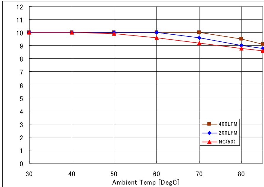
Fig-1.8V-1: Available load current vs. ambient temperature and airflow rates for Vout=1.8V with Vin=12.0V. Maximum component temperature \leq 120°C
