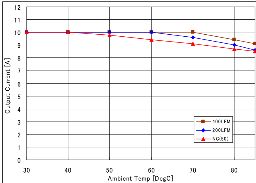
Fig-2.0V-1: Available load current vs. ambient temperature and airflow rates for Vout=2.0V with Vin=12.0V. Maximum component temperature \leq 120°C
