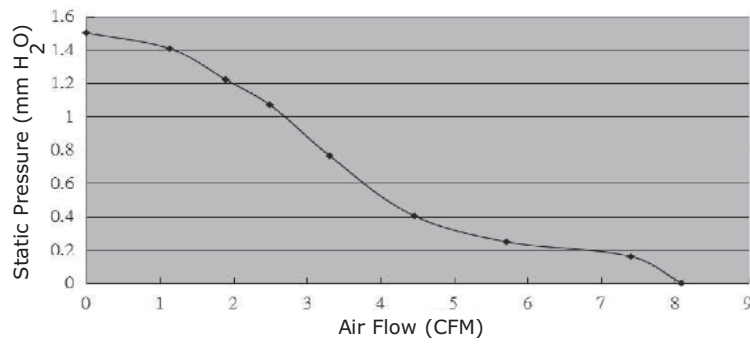
CFM-5020B-130-235
