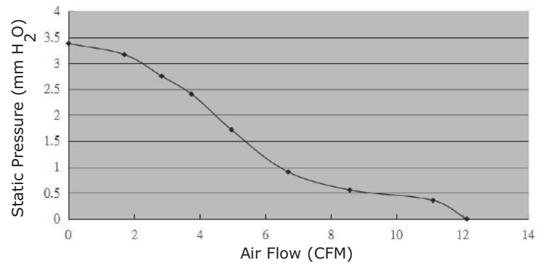
CFM-5020B-145-323
