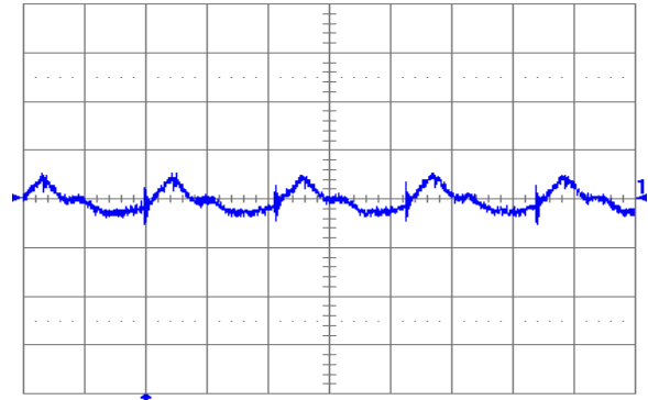
Fig. 2.5V.6: Output voltage ripple (20 mV/div.) at full rated load current into a resistive load with external capacitance 47\text{ }\mu\text{F} ceramic + 1\text{ }\mu\text{F} ceramic, and V_{in} = 12\text{ V} for V_{out} = 2.5\text{ V} . Time scale: 1 \mu\text{s} /div.
