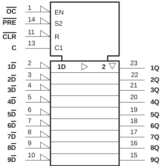
logic symbol†
