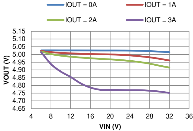
Figure 26. Line Regulation
