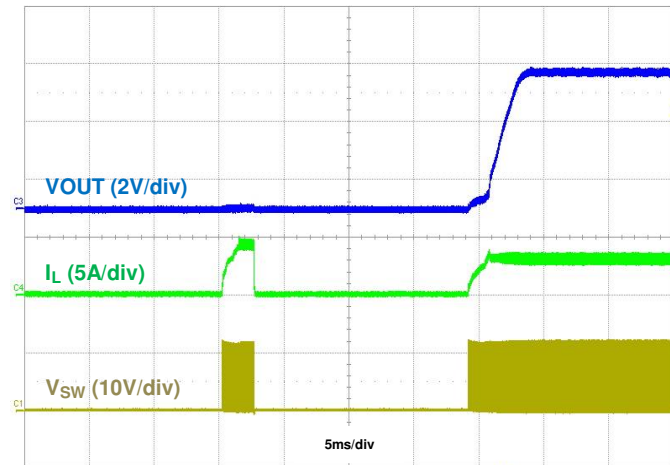
Figure 11. Output Short Recovery, IOU = 3A
