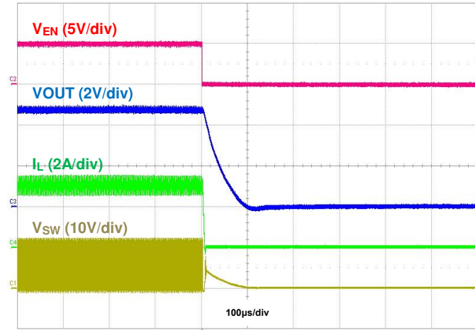
Figure 9. Shutdown using EN, IOU = 3A
