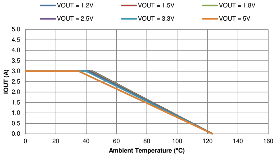
Figure 38. Output Current Derating Curve vs. Ambient Temperature, VIN = 12V
