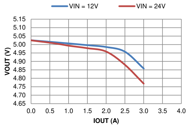
Figure 27. Load Regulation
