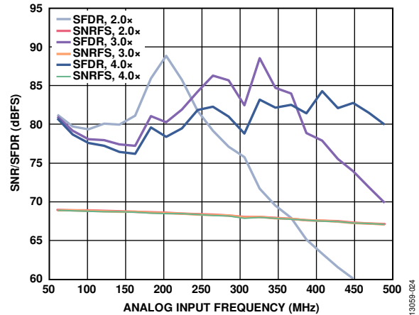
Figure 25. SNR/SFDR vs. Analog Input Frequency ( f_{IN} ); f_{IN} < 500\text{ MHz} ; Buffer Control 1 Setting = 2.0\times , 3.0\times , and 4.0\times
