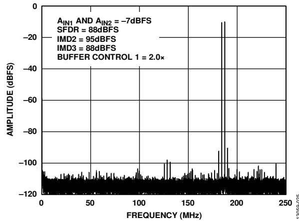
Figure 26. Two-Tone FFT; f_{IN1} = 184\text{ MHz} , f_{IN2} = 187\text{ MHz}
