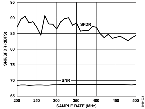
Figure 24. SNR/SFDR vs. Sample Rate ( f_s ); f_{IN} = 170.3\text{ MHz}
