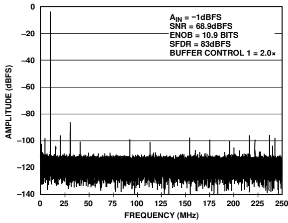
Figure 15. Single-Tone FFT with f_{IN} = 10.3 MHz
