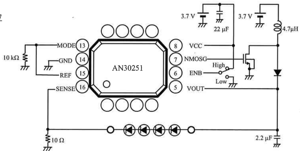
Test Circuit 7
