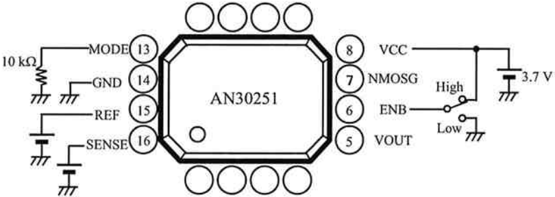
Test Circuit 3
