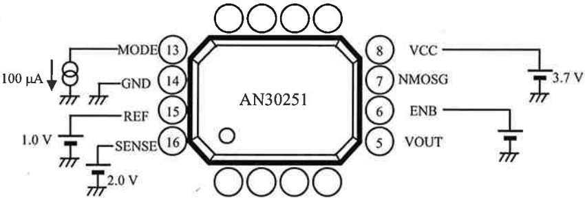
Test Circuit 2
