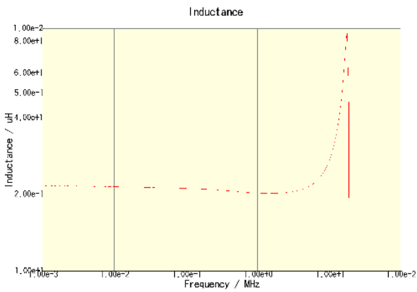
CLF6045T-220M-CA
