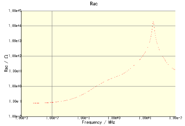
CLF6045T-220M-CA
