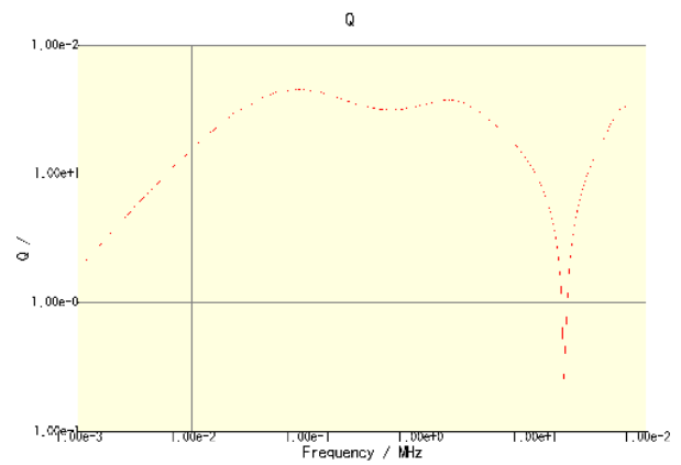
CLF6045T-220M-CA
