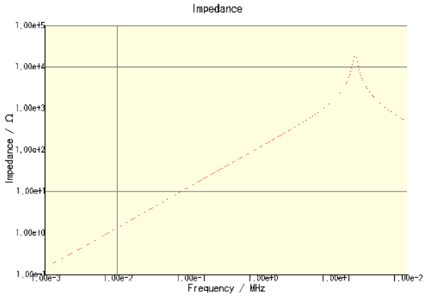
CLF6045T-220M-CA
