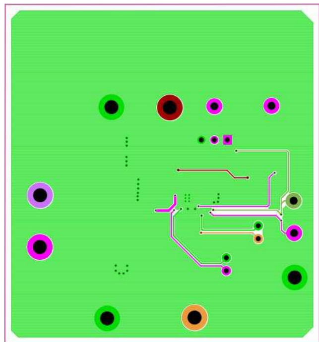
Figure 8. Bottom Layer
