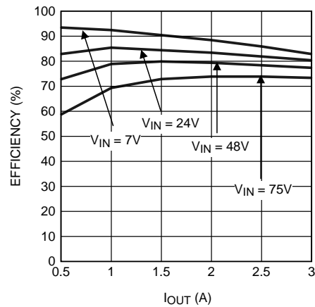
Figure 9. Demoboard Efficiency vs I_{OUT} and V_{IN}
