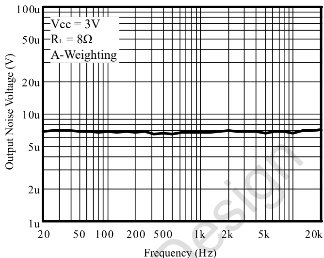
Figure 15 Noise Floor
