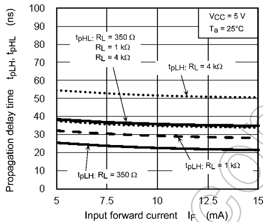
Fig. 12.2.15 t_{pLH}, t_{pHL} - I_F
