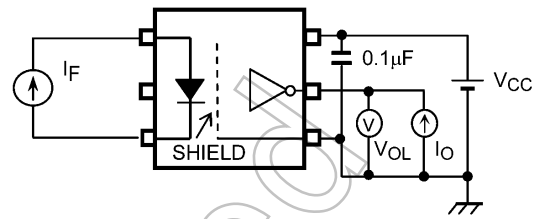
Fig. 12.1.2 V_{OL} Test Circuit
