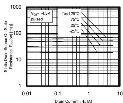
Fig.3 Static Drain-Source On-State Resistance vs. Drain Current (2)
