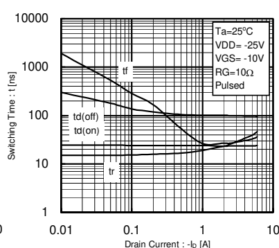
Fig.8 Switching Characteristics
