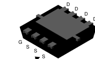
Bottom View Pin 1
